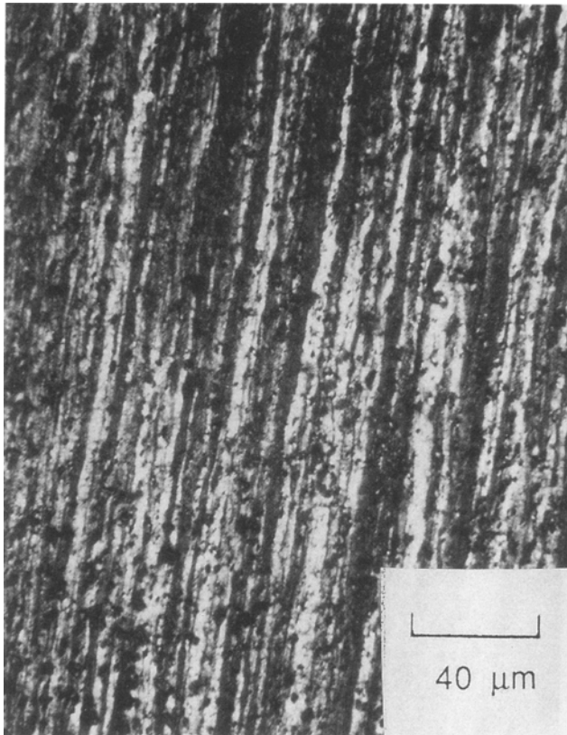
Fig. 10 The grain and particle structure of E3 as finally rolled to 0.33 mm
