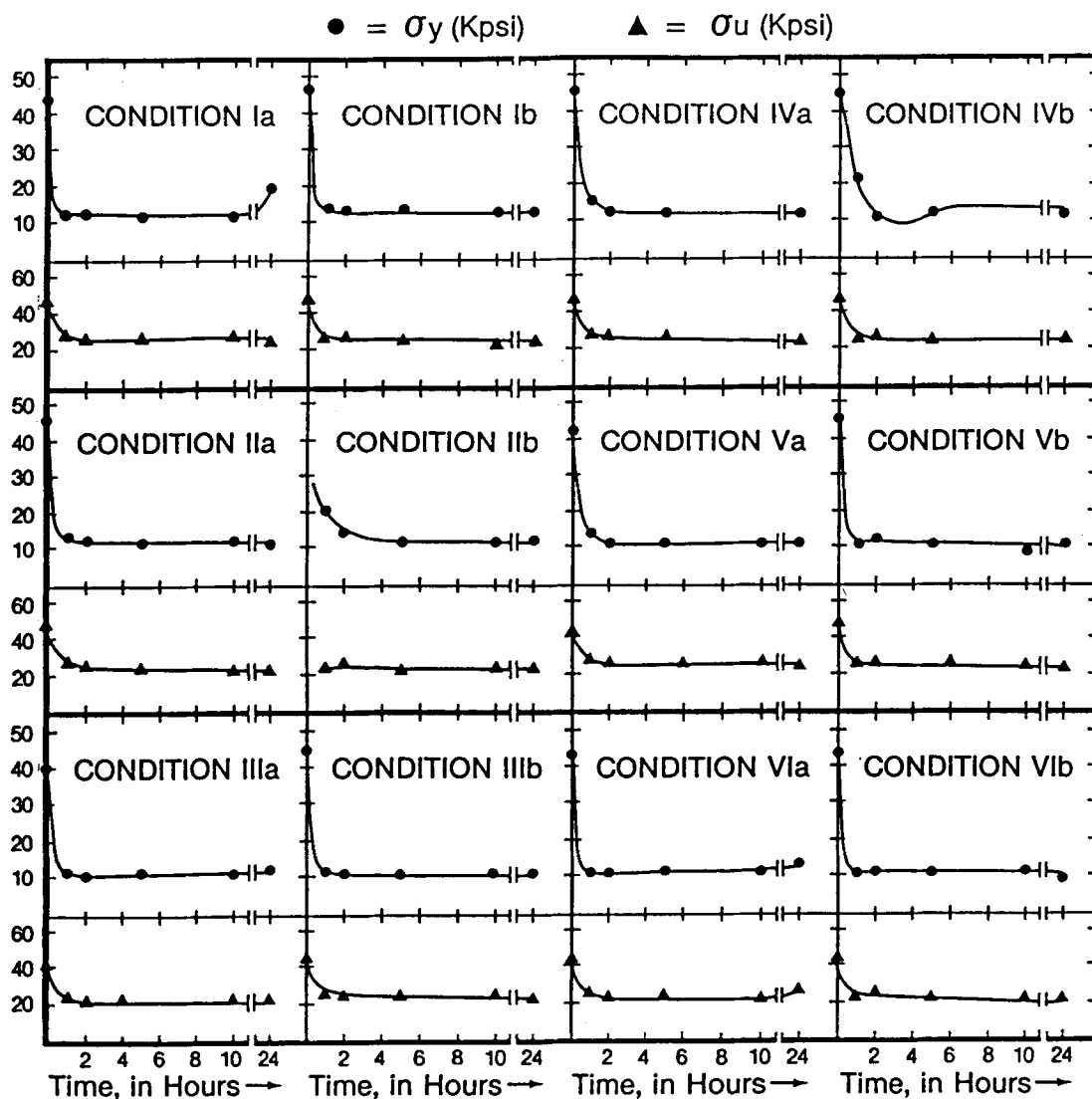
Fig. 4 Yield stress and ultimate tensile stress changes versus annealing time. 1 ksi = 6.89 MPa
