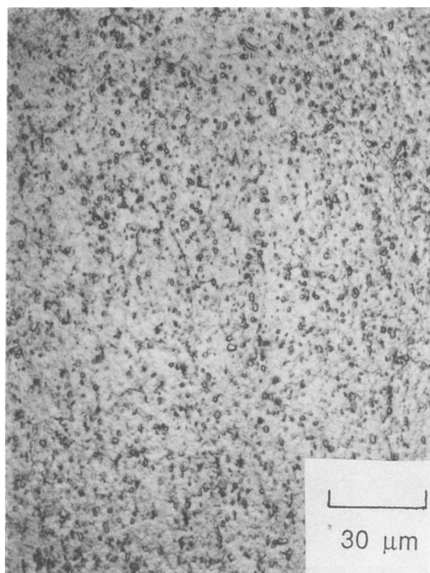
Fig. 6 Grain structure and particle structure of type 3004 aluminum alloy at two magnifications. Both images are in Condition I, as recrystallized (454 °C/24 h) after 95% cold work.
