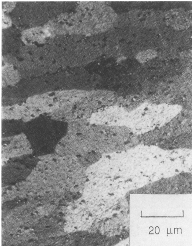
Fig. 8 The grain structure of E1 as recrystallized
