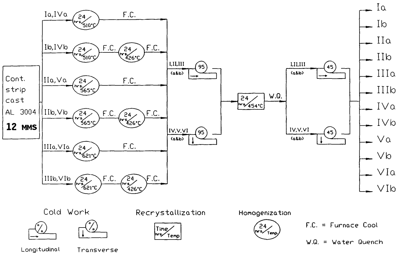
Fig. 1 Thermomechanical process to study the effect of homogenization treatments on the mechanical anisotropic behavior of AA 3004 strip cast aluminum alloy
