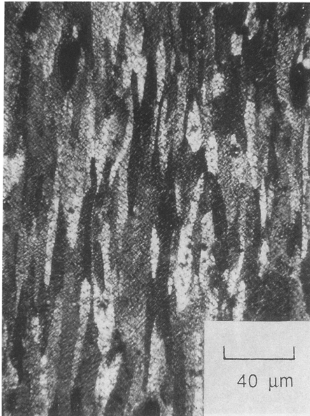
Fig. 7 Grain and particle structure of condition I as finally rolled (45% cold work) to 0.33 mm
